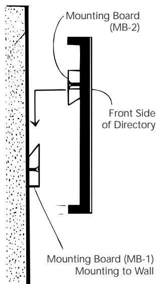
Wall Mount
